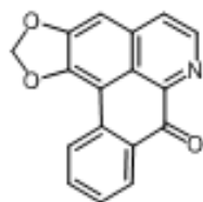
Figure 6. Liriodenine
