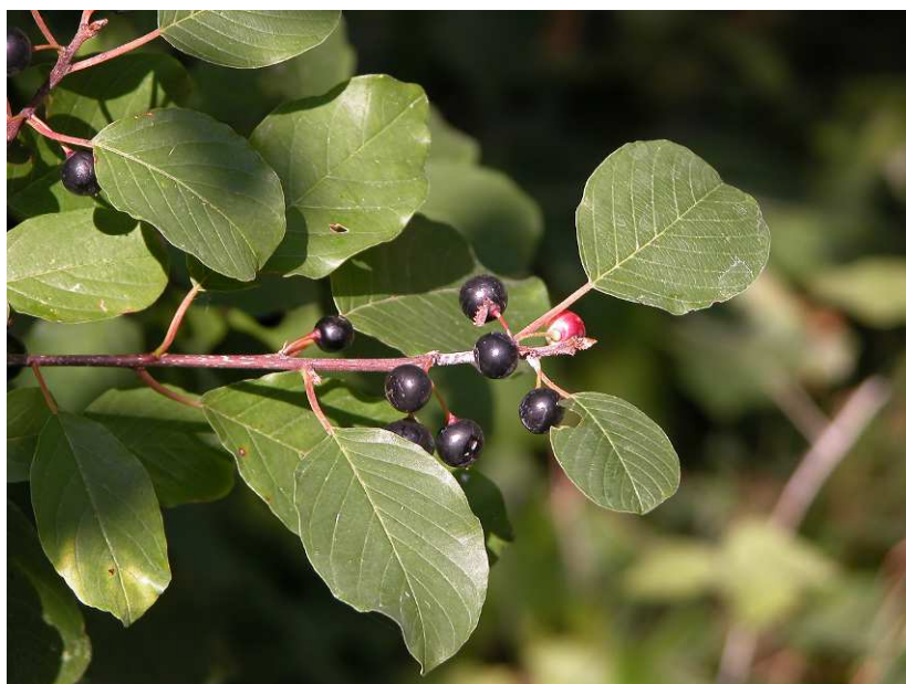
Figure 11. Rhamnus frangula
