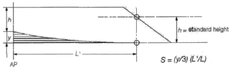
Fig. 3 Sheer credit S for excess height
