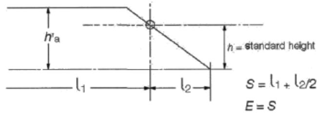
Fig. 2 Height of superstructure greater than the standard height
