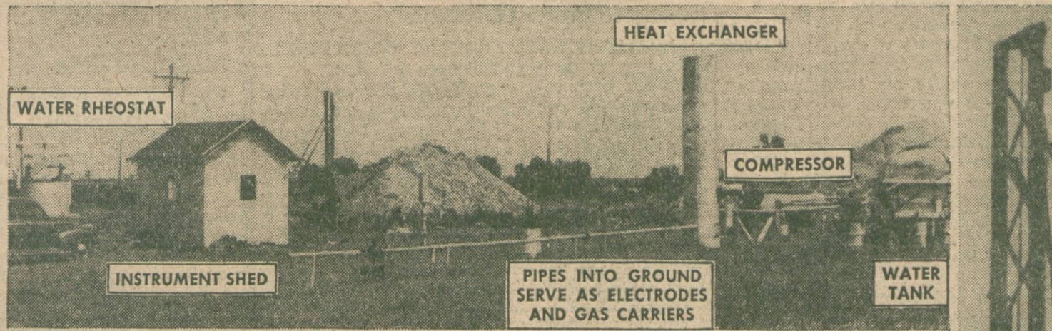
Rheostat controls amount of current going into electrodes to generate gas underground. Gas passes through exchanger.
