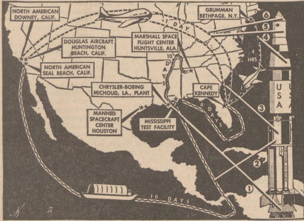
SATURN HAUL PATTERN—Here is a diagrammatic picture of how the giant Saturn rockets and Apollo spacecraft are moved to Cape Kennedy from widely scattered production plants and test sites.
