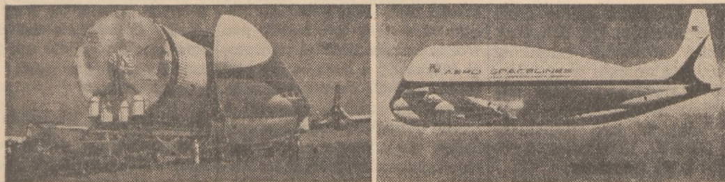
A stage of an Apollo being loaded into a Super Guppy, and the big fat plane in flight.
