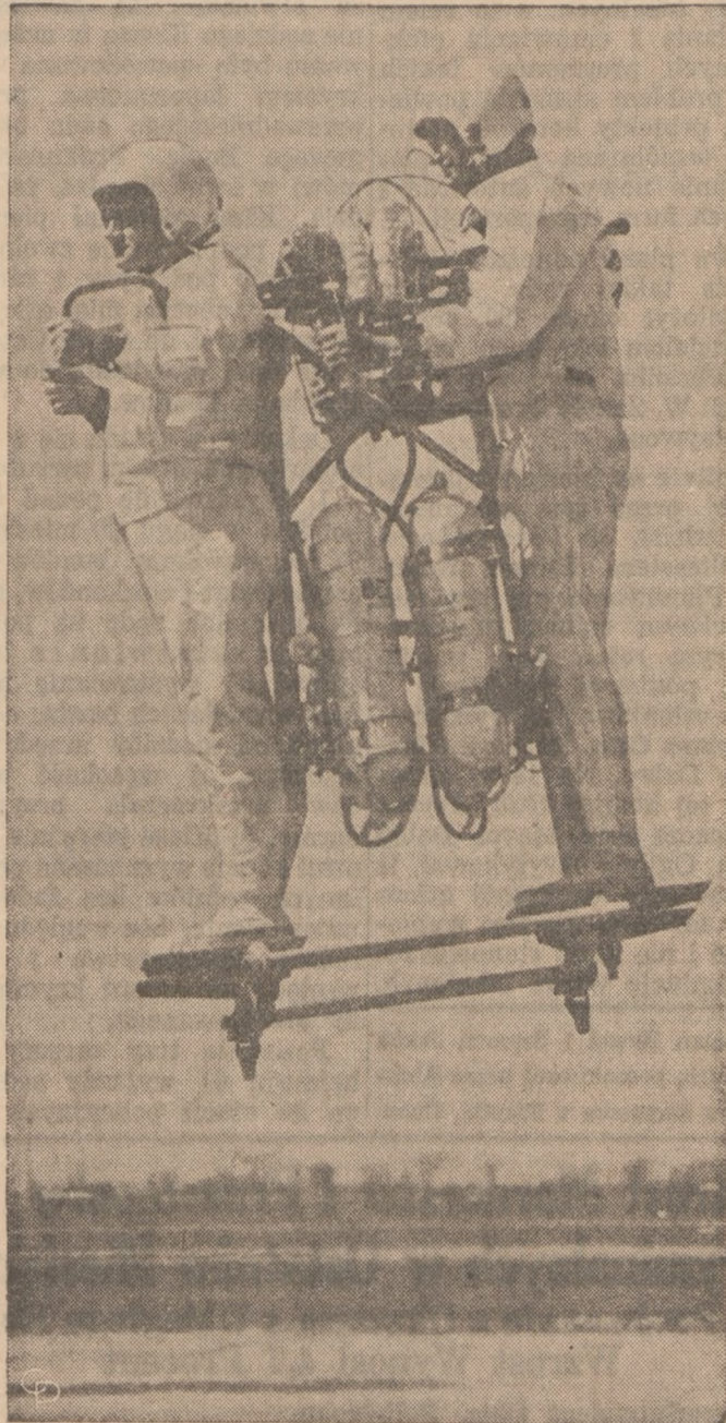
TWO-MAN ROCKET PASSES TEST—A two-man rocket system called Pogo that could provide taxi service for astronauts on a lunar probe, or rescue stranded mountaineers, hovers above the ground during a successful test at the Bell Aero Systems Company in Buffalo, N.Y.
