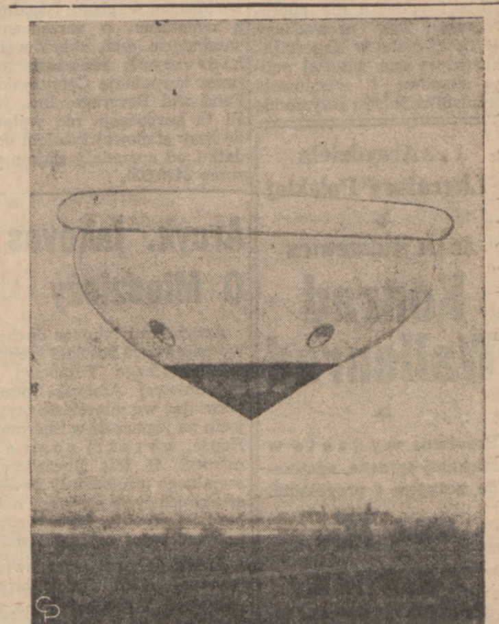
SPACE BRAKE TESTED—A space brake made by Goodyear Aerospace Corp. at Akron, Ohio, that may be a forerunner of a device to slow spacecraft for soft landing on Mars, makes a successful drop with a Mars Lander at Wallops Island, Va. The air-filled ballute (balloon-parachute) measures 21 feet high and 37 feet in diameter. Its "portholes" are vents which admit air to keep the device inflated.
