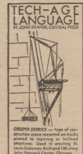
CREEPER DERRICK - type of construction crane mounted on tracks pinned to tapering or inclined structures. Used in erecting St. Louis Gateway Arch and 100-story John Hancock Center, Chicago.
