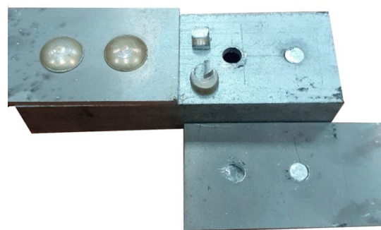
Fig. 13. Nature of fatigue failure of rivets of a single-strap sample with C-profile
