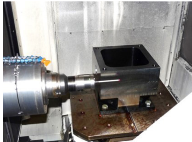
Fig. 5. View of the rectangular master part with the RMP60 object probe placed in a 4-axis horizontal machining center
