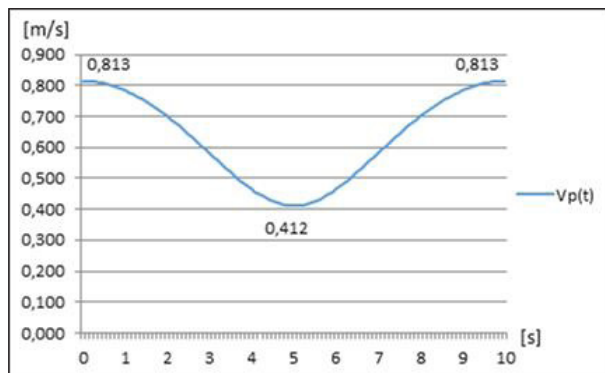
Fig. 5. Values of the instantaneous lapping speed in a system of a standard single-disc lapping machine for: a) r = 40 mm, b) r = 30 mm, c) r = 20 mm, d) r = 10 mm ( R = 65 mm, \omega_t = 3\pi rad/s, \omega_2 = 0,2\pi rad/s)
