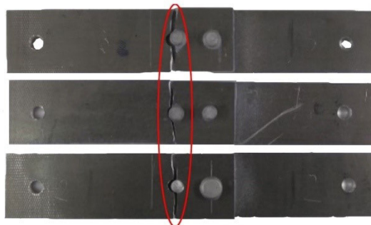
Fig. 7. Fatigue destruction of riveted single-overlap samples [1]
