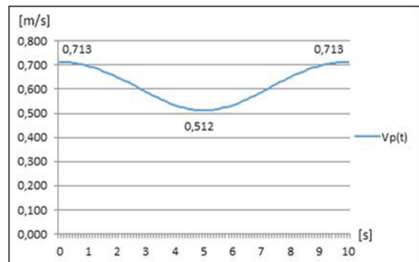
Fig. 5. Values of the instantaneous lapping speed in a system of a standard single-disc lapping machine for: a) r = 40 mm, b) r = 30 mm, c) r = 20 mm, d) r = 10 mm ( R = 65 mm, \omega_t = 3\pi rad/s, \omega_2 = 0,2\pi rad/s)
