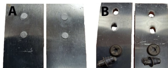
Fig. 2. Destruction of standard and blind rivets in the static strength test
