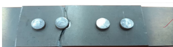
Fig. 11. Fatigue crack of flat cover plate
