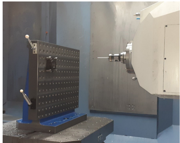
Fig. 7. View of the calibration master (two reference sphere's, calibration column), together with the RMP60 probe, inside 5-axis machine center
