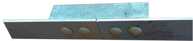
Fig. 12. Single strap sample with C-profile
