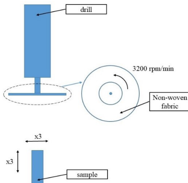
Fig 1. Diagram of processing of EN AW-2017A aluminum alloy samples
